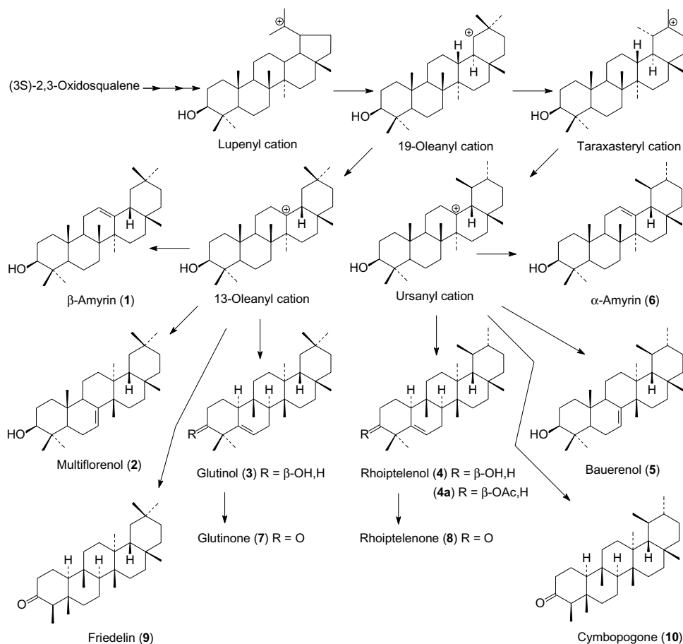
Fig. 1. Biosynthesis of pentacyclic triterpenes.
